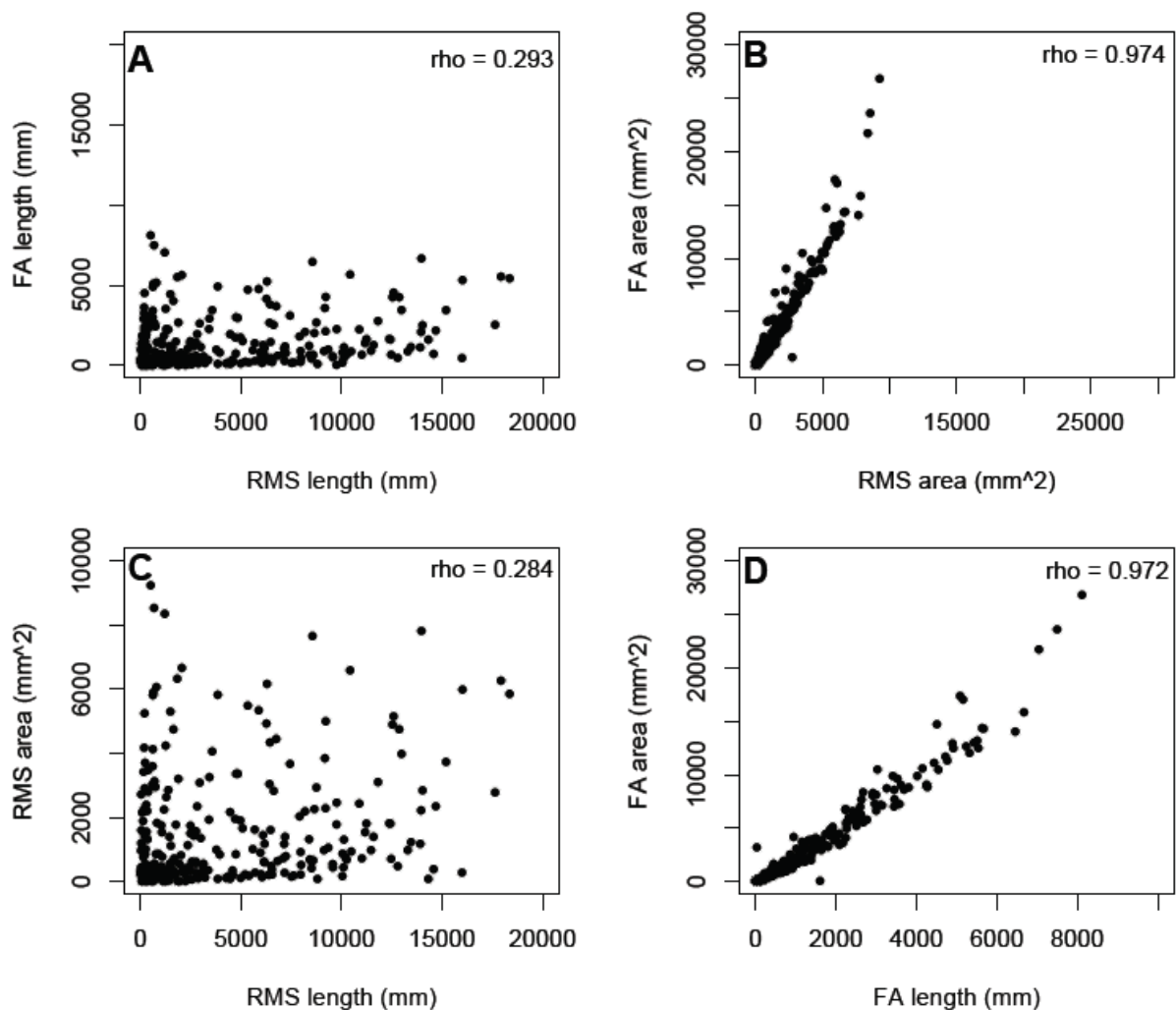
Fig. 3. Scatterplots with Spearman rank order correlation coefficients ( \rho ) for relationships between Root Measurement System (RMS) and Feature Analyst (FA) measures of root length and root area.
